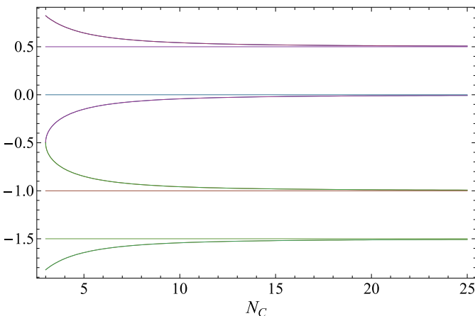
Fig. 1. N_c dependence of the eigenvalues of the model \text{TOY}_{\text{Adj,Fund}}
